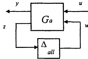
Fig. 5 Extended LFT representation for robust performance.
