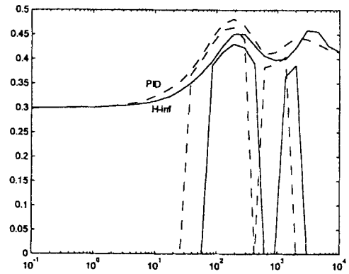
Fig. 6 Structured singular value for robust stability
