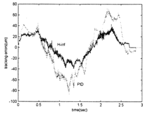
(b) Errors for the Y axis
