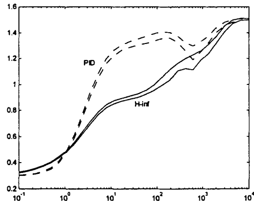
Fig. 7 Structured singular value for robust performance.
