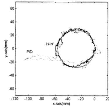
(c) Errors for the circle
