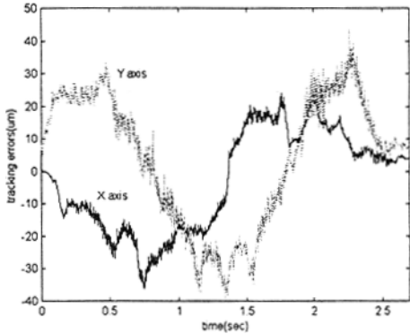
Fig. 10 Tracking errors for the MIMO controller.
