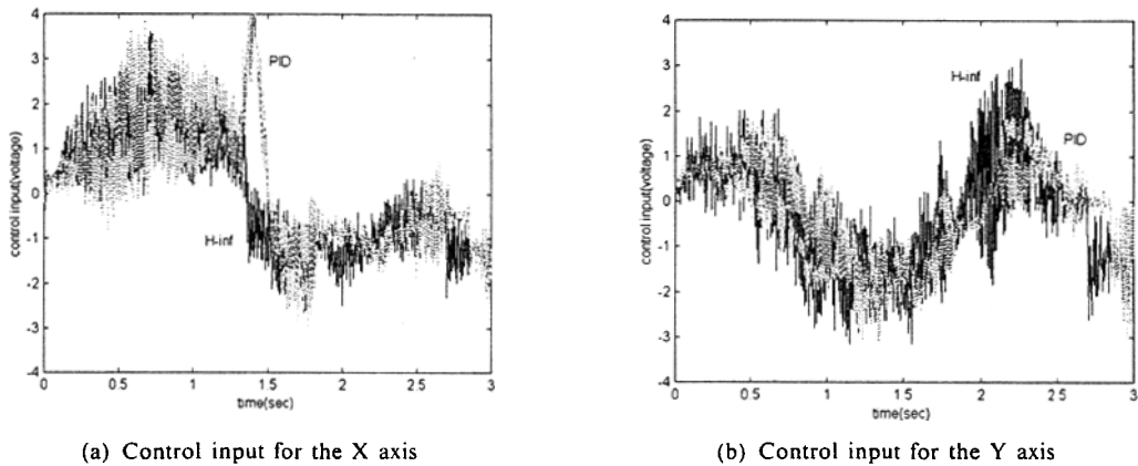
Fig. 13 Comparison of the control inputs.
