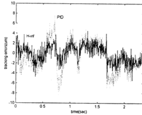
(b) Errors for the Y-axis
