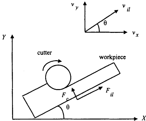
Fig. 1 Cutting forces applied to a workpiece.
