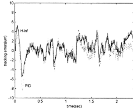
(a) Errors for the X-axis
